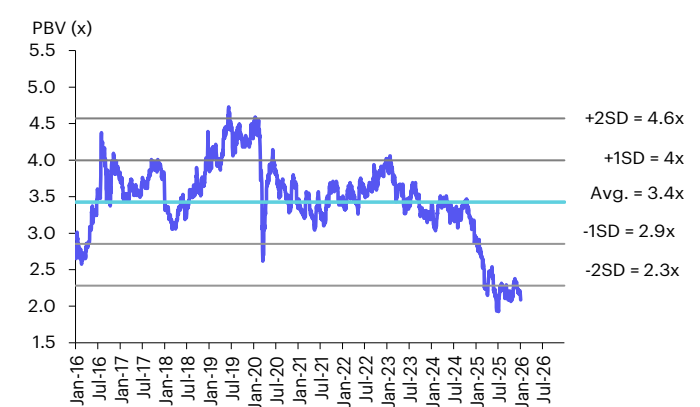
Figure 5: PBV Band
