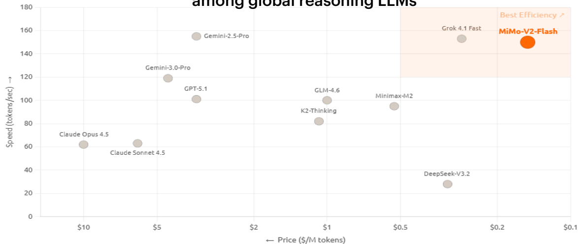
MiMo-V2-Flash achieves low token cost but high inference speed among global reasoning LLMs
