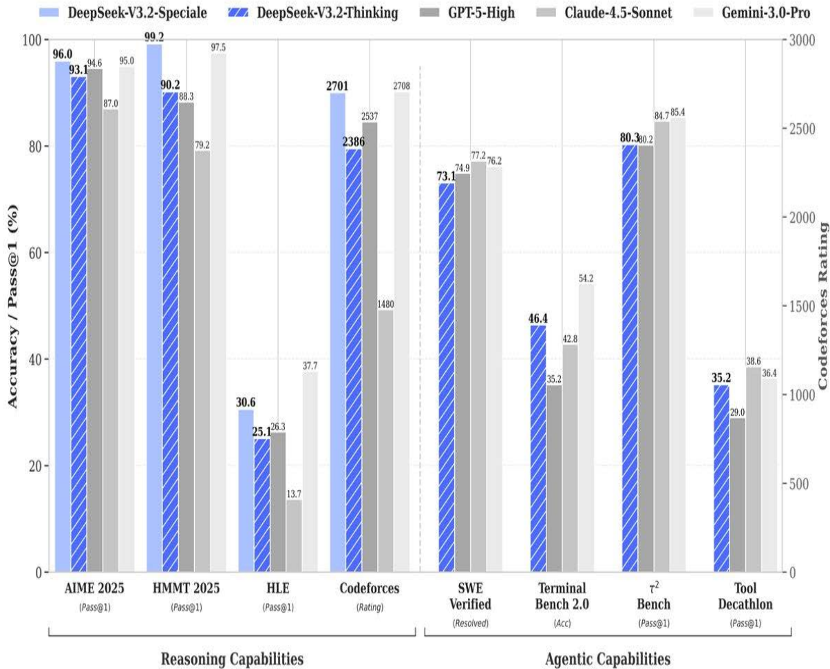
AI Model Performance Comparison: Reasoning and Agentic Capabilities
