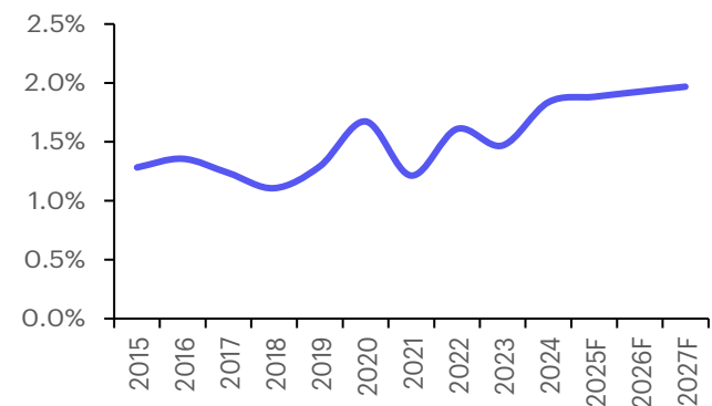
Figure 5: NPL ratio
