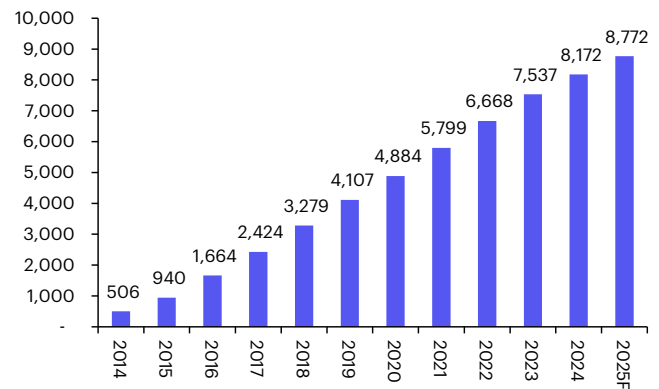
Figure 2: Branches
