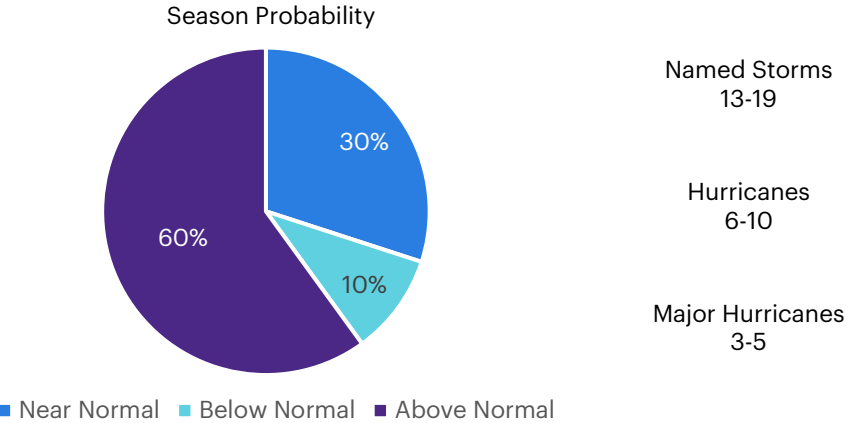
Figure 7: Atlantic Expecting Above Normal Hurricane Season
