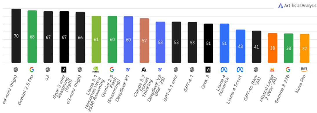
Artificial Analysis Intelligence Index Intelligence Index incorporates 7 evaluations: MMLU-Pro, GPQA Diamond, Humanity's Last Exam, LiveCodeBench, SciCode, AIME, MATH-500
