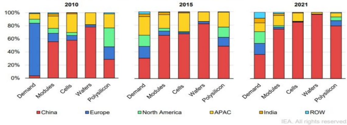
Solar PV manufacturing capacity by country and region, 2010-2021
