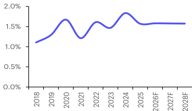
Figure 5: NPL ratio
