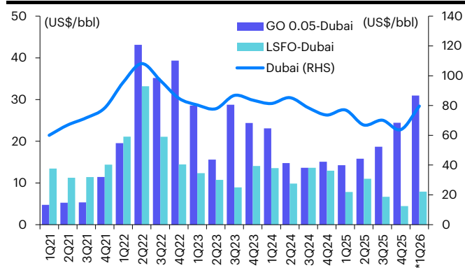
Figure 1: Crack spread – Gasoil and LSFO
