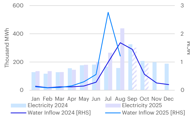
Figure 4: NN2 Electricity Generation Accelerated
