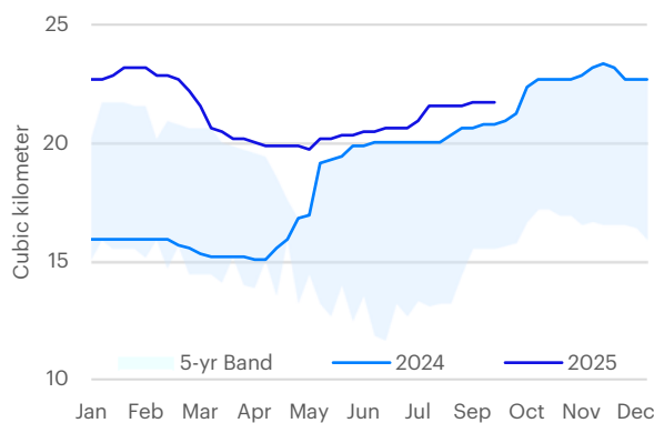
Figure 3: Nuozhadu's Level Remained above 5-yr High
