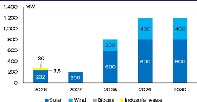
Figure 2: SCOD for first round of phase 2 renewable bidding under FiT scheme
